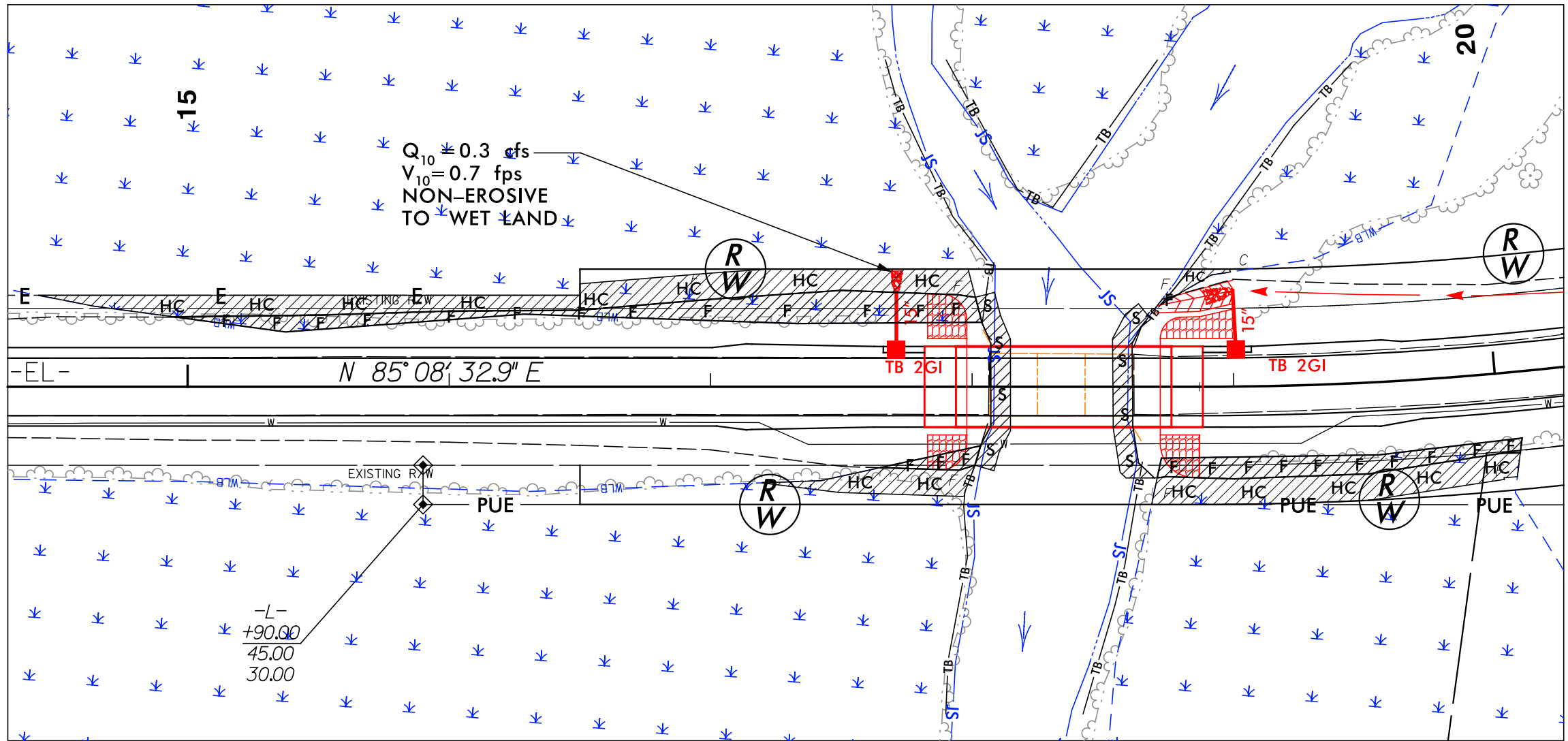
ENLARGED PLAN VIEW SITE 1
