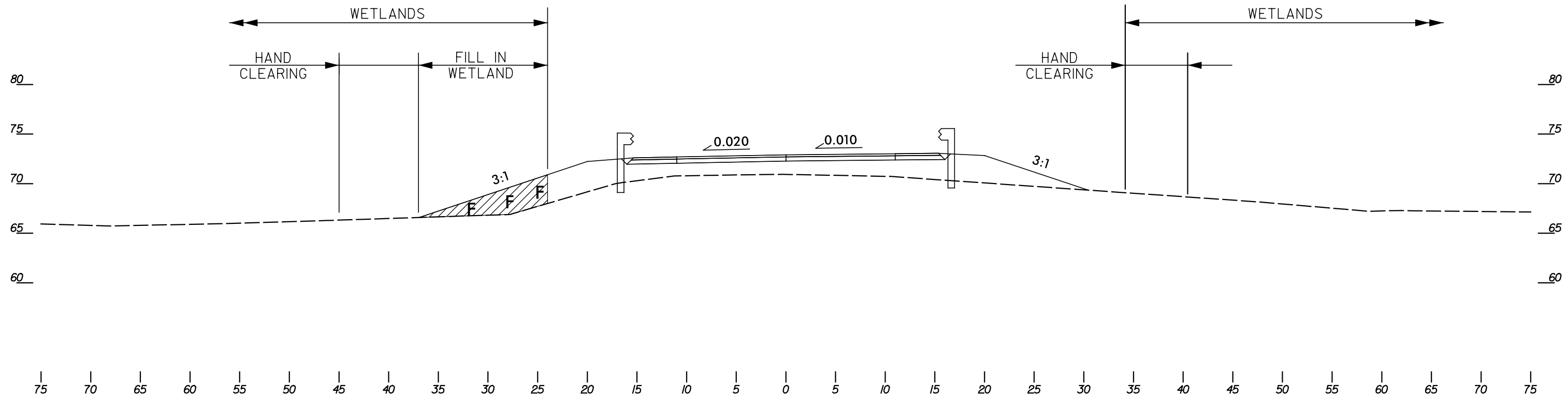
SITE I X-SECTION STA 17+50 -L-
